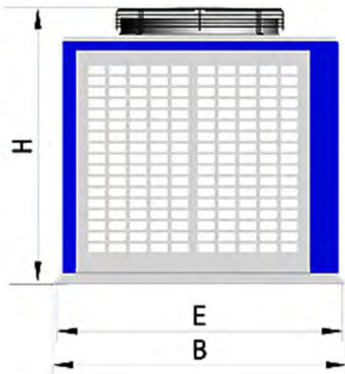
Condenser performance & Overall Dimension
