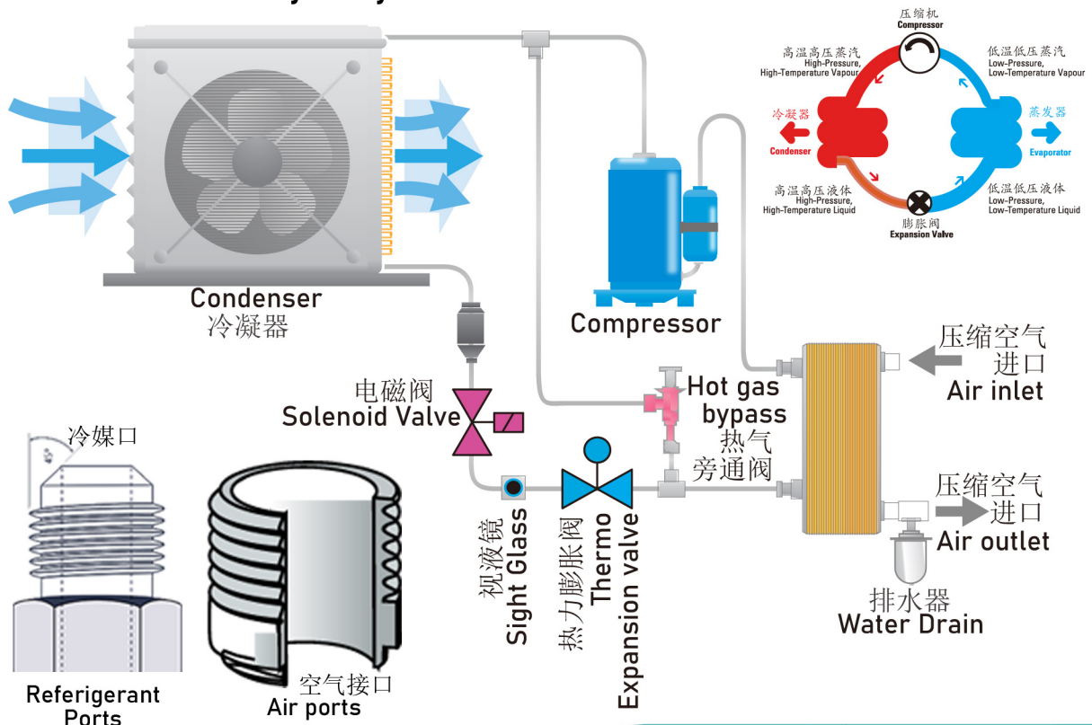
Air cooled air dryer system chart
